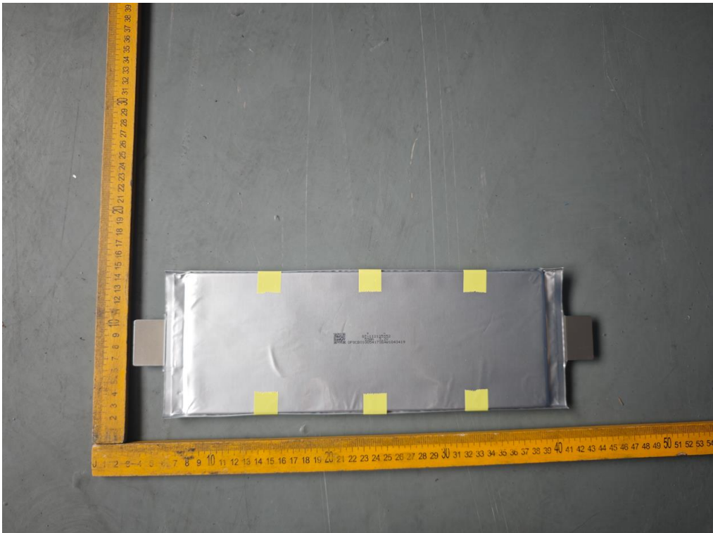
Figure 3 Overall view of cell (电芯外观图)
